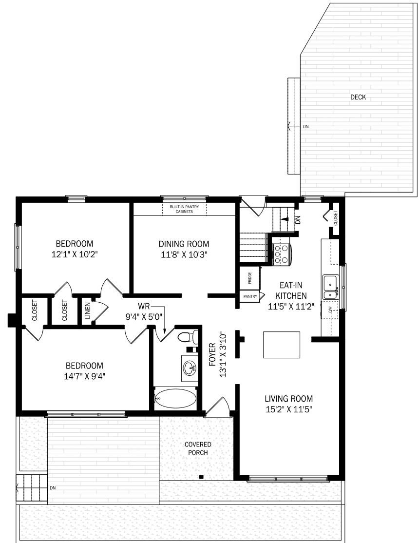
MAIN FLOOR - 1030 SQUARE FEET
